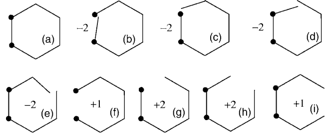
FIG. 21. Susceptibility hexagons on either H or B lattice.
