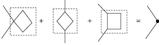
FIG. 15. The factors associated with the dashed box in the first three diagrams renormalize the vertex (the filled circle) in the last diagram. We label these contributions SQ1, SQ2, and SQ3, respectively.
