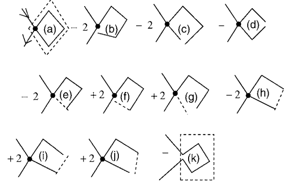
FIG. 16. Diagrams for square SQ1 of 15 on either H or B lattice. Diagram (k) occurs on the Bethe lattice but must be subtracted off because its counterpart on the hypercubic lattice has a different topology.
