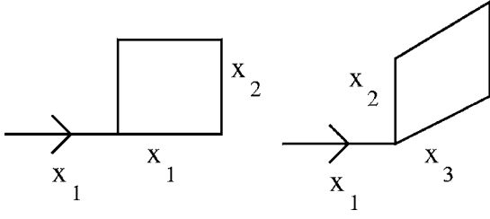
FIG. 9. Attaching a square to a site.
