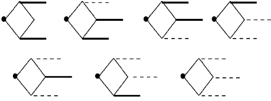
FIG. 11. Configurations of diagram (a) of Fig. 7 which have two paths to infinity. The heavy line is a bond which is (k-1) -connected to infinity and carries a factor P^{\sigma-1} . The dashed line carries a factor R_{k-2} which may survive culling if it is connected to two live bonds.
