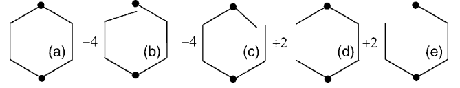
FIG. 23. Susceptibility hexagons on either H or B lattice.
