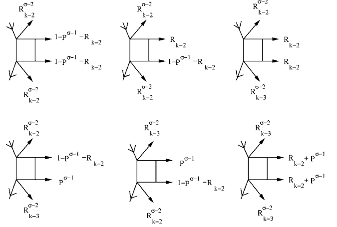
FIG. 20. Evaluation of \Delta R(a) of Eq. (99).
