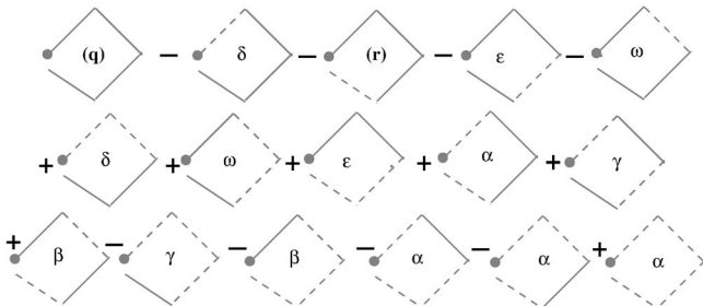
FIG. 6. As above, but for the B lattice.
