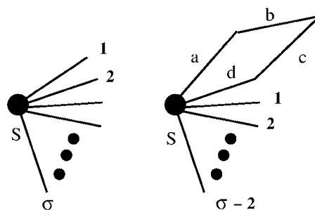
FIG. 2. Diagrammatic representation of the EOS. Left: the unperturbed EOS based on a seed site, S , with \sigma emerging bonds. Right: the perturbation to the EOS from the insertion of a square, so that now the seed site has \sigma-2 single bonds and an attached square.
