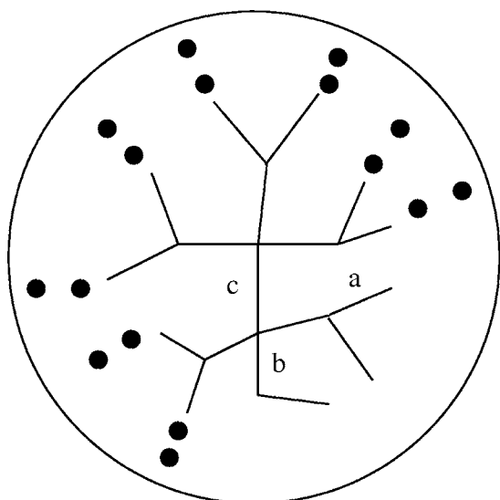
FIG. 1. Culling of a cluster for k=3 on a Bethe lattice with coordination number z=4 . The filled circles indicate branches which are k-1 connected to infinity. Culling removes the bonds at a , b , and eventually at c , including the lower two sets of filled circles, but the rest of the cluster survives.
