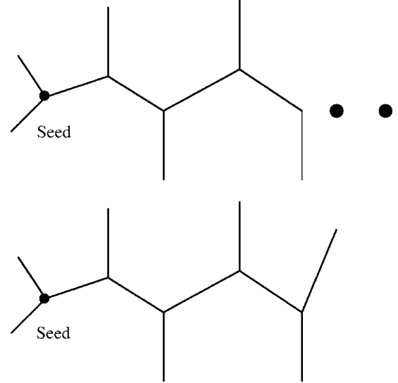
FIG. 14. Configurations for k=3 illustrating “truncation” of diagrams. Here the side branches are assumed to be (k-1) -connected to infinity. In the top panel a configuration is shown where the k -core depends on the state of the further bonds indicated by filled circles. In the lower panel, the configuration is (k=3) -connected no matter what happens further down the chain. Since the k -core does not depend on further bond occupation probabilities this diagram cannot be extended.
