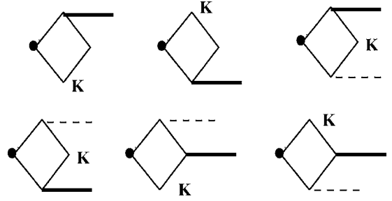
FIG. 12. As in Fig. 11, configurations of diagram (a) of Fig. 7 which have one path to infinity. The symbol K denotes a bond which is definitely culled and therefore carries a factor (1 - P^{\sigma-1} - R_{k-2}) .
