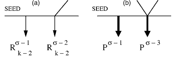
FIG. 10. Definition of R_k^{\sigma-m} (a) and P^{\sigma-r} (b). Each site has \sigma+1 bonds.
