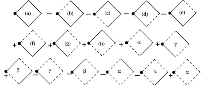
FIG. 3. Contributions from the 16 subdiagrams [of diagram (a)] which result from either occupying (full line) or not occupying (dashed line) each bond of the square on the H lattice. Greek letters label sets of subdiagrams which cancel one another.
