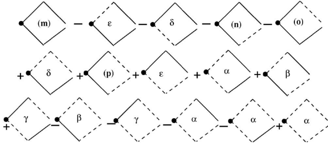
FIG. 5. As above, but for the B lattice.
