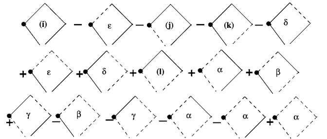
FIG. 4. As above, but for the B lattice. Vertices which are close to one another would coincide on the H lattice.
