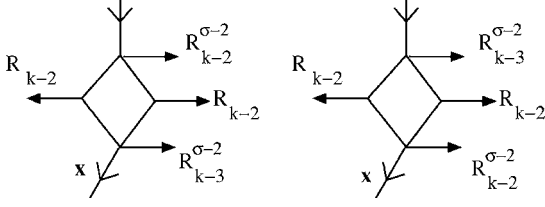
FIG. 19. Diagrams for Eq. (92). In the left-hand diagram the bottom site will be culled if the bond x is culled. In that case the entire cluster will be culled. So the stability of this cluster depends on the state of bonds below x , and therefore this diagram can be extended. In contrast, the right-hand cluster survives culling no matter what may be the state of bond x . Hence this diagram truncates and we discard it.
