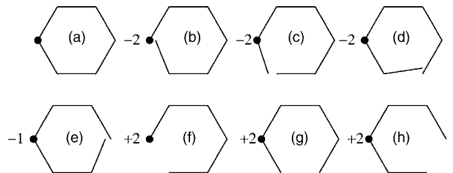
FIG. 8. As in Fig. 7, contributions to \Phi(Q) from hexagons on either a H or a B lattice. Diagrams (f), (g), and (h) correspond to sums of graphs on both the H and B lattices. For example, the square equivalent to hexagon diagram (f) is the sum of diagrams (b), (r), and (j) in Fig. 7. Diagrams similar to these give the contribution to the susceptibility, \Gamma_{H,A} , due to hexagon insertions as we will eventually show.
