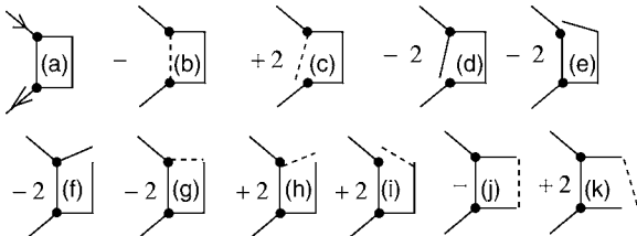
FIG. 18. Diagrams for square SQ3 of 15 on either H or B lattice.
